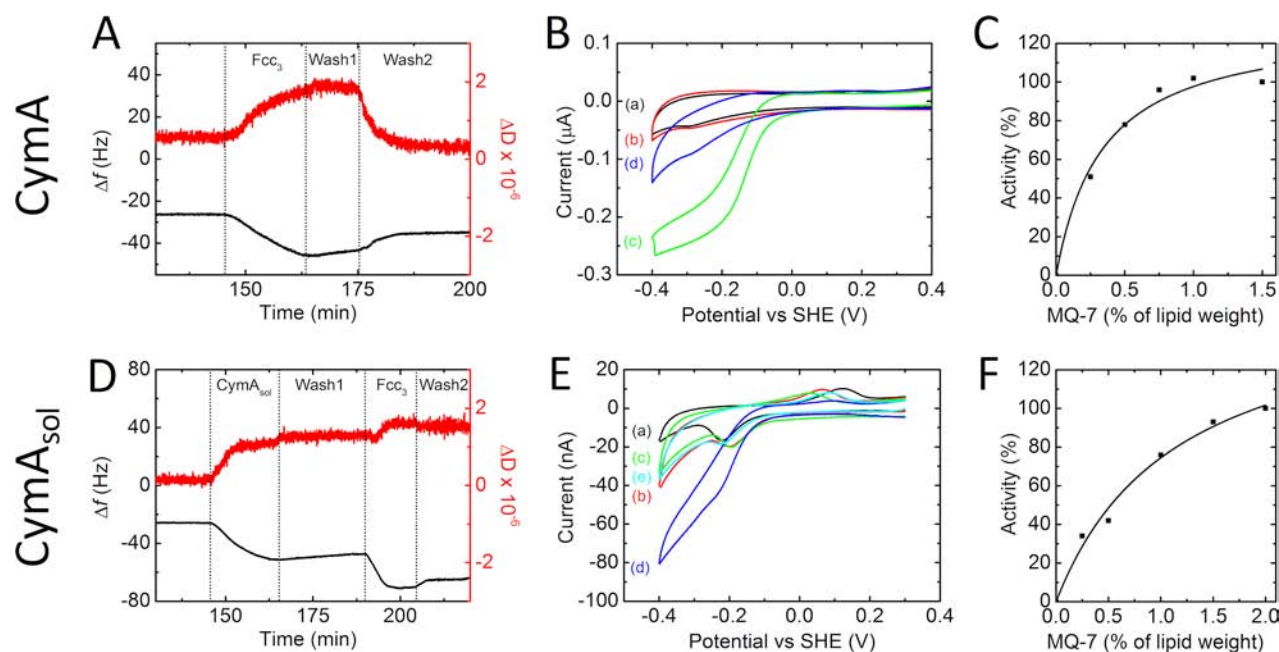
Figure 2. The assembly and catalytic activities of \text{CymA}_{(\text{sol})} containing SSMs. (A) QCM-D results of a \text{SiO}_2 surface in buffer, plotting (black line, left axis) frequency and (red line, right axis) dissipation against time. For clarity, only the results after formation of the SSM are shown. Changes in the solution composition flowing over the SSM are indicated: ( \text{Fcc}_3 ) 5 \mu\text{M} \text{Fcc}_3 /1 mM fumarate; (wash 1) 1 mM fumarate; (wash 2) buffer only. SSM was formed with CymA proteoliposomes (90:10 POPC:cardiolipin; 2% (w/w) CymA; 1% (w/w) MQ-7). The plot shown is representative of triplicate experiments. (B) CVs (10 mV/s) of a SSM on a gold electrode modified with cholesterol tethers. The SSM was formed with CymA proteoliposomes (90:10 POPC:cardiolipin; 1% (w/w) CymA; 1% (w/w) MQ-7). CVs are shown (a) before and after addition of (b) 5 \mu\text{M} \text{Fcc}_3 , (c) 1 mM fumarate (after rinsing unbound \text{Fcc}_3 from solution), and (d) 1 mM fumarate/10 \mu\text{M} HQNO. (C) Relative current measured from CVs as in (B, trace c) at -0.25 V vs SHE of the reductive scan as a function of MQ-7 concentration in the SSM. MQ-7 content is given in weight percentages relative to the lipid weight in the proteoliposomes. The line represents a fit to the Michaelis–Menten equation. (D) QCM-D results of a \text{SiO}_2 surface in buffer, plotting (black line, left axis) frequency and (red line, right axis) dissipation against time. For clarity reasons, only the traces after the formation of the SSM are shown. Changes in the solution composition flowing over the SSM are indicated: ( \text{CymA}_{(\text{sol})} ) 0.1 \mu\text{M} \text{CymA}_{(\text{sol})} ; (wash 1), 1 mM fumarate; ( \text{Fcc}_3 ) 5 \mu\text{M} \text{Fcc}_3 /1 mM fumarate; (wash 2) 1 mM fumarate. SSM was formed with liposomes (90:10 POPC:cardiolipin; 1% (w/w) MQ-7). The plot shown is representative of triplicate experiments. (E) CVs (1 mV/s) of a SSM on a gold electrode modified with cholesterol tethers. The SSM was formed with liposomes (90:10 POPC:cardiolipin; 2% (w/w) MQ-7). CVs are shown (a) before and after addition of (b) 0.1 \mu\text{M} \text{CymA}_{(\text{sol})} , (c) 5 \mu\text{M} \text{Fcc}_3 , (d) 1 mM fumarate (after rinsing unbound \text{Fcc}_3 from solution), and (e) 1 mM fumarate/10 \mu\text{M} HQNO. (F) Relative current measured from CVs as in (E, trace d) at -0.25 V vs SHE of the reductive scan as a function of MQ-7 concentration in the SSM. MQ-7 content is given in weight percentages relative to the lipid weight in the liposomes. The line represents a fit to the Michaelis–Menten equation.
